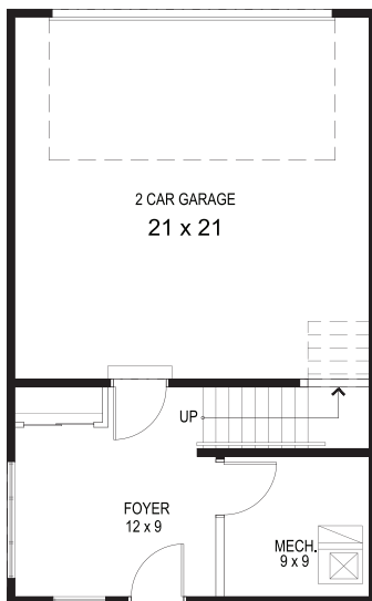
MAIN FLOOR
