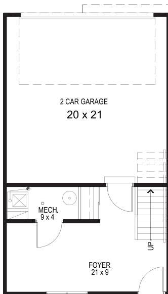
MAIN FLOOR
